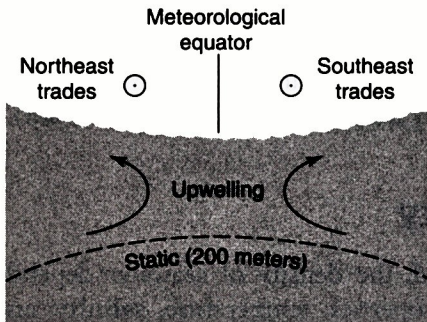
c Open-ocean Coriolis-effect equatorial upwelling
