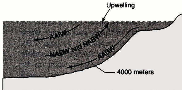
d Density-driven upwelling
