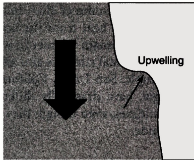
b Obstruction upwelling
