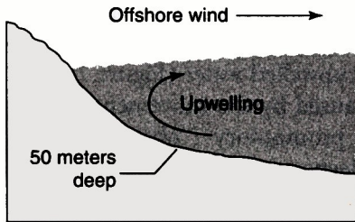
a Wind-driven upwelling
